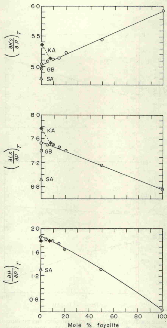
FIG. 3. Pressure derivatives of compressional modulus L_s , shear modulus \mu , and the adiabatic bulk modulus K_s of olivine as a function of (Fe/Mg) ratio; comparison with literature data. ( \Delta ) indicates the datum of Schreiber & Anderson (SA, 1967), ( \square ) indicates the datum of Graham & Barsch (GB, 1969), and ( \blacklozenge ) indicates the data points of Kumasawa & Anderson (KA, 1969); ( \circ ) are the present work.
